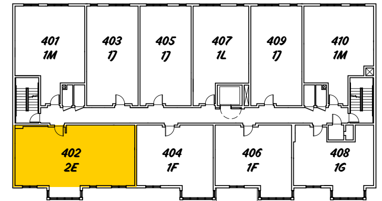
4TH FLOOR
